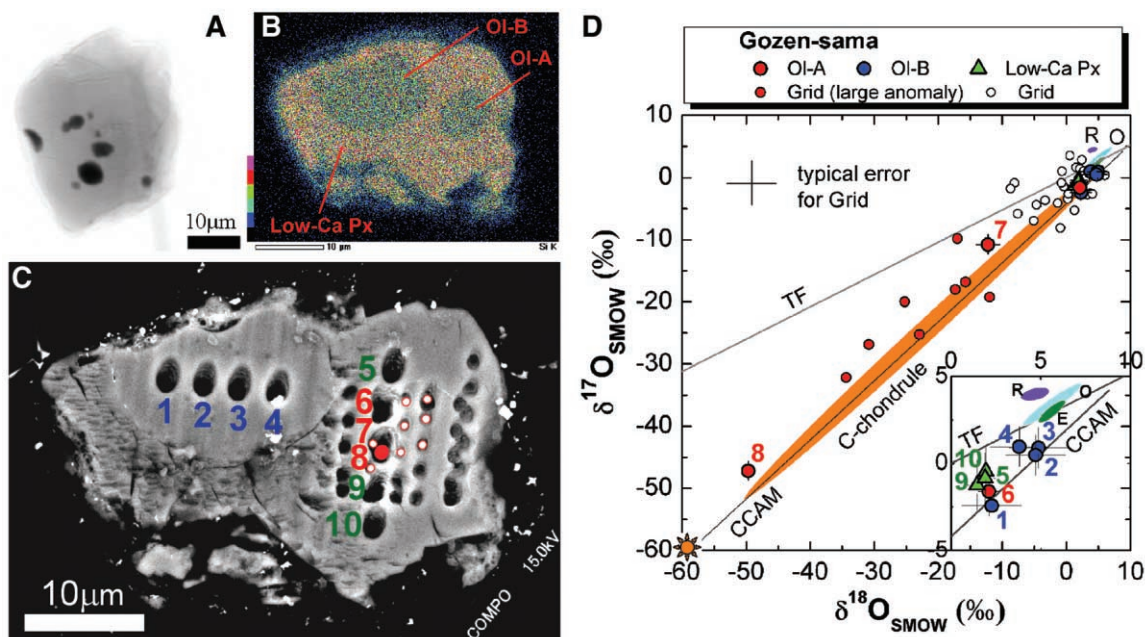
Fig. 2. A large terminal particle, Gozen-sama, 40 \mu\text{m} in diameter.
